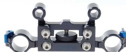
Adaptor 401-17 for 19mm rods with horizontally and vertically adjustable mounts for 15mm rods
