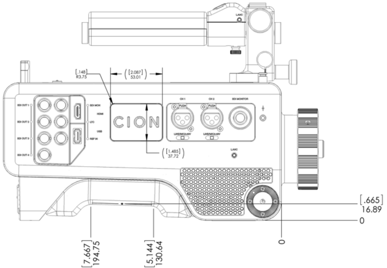
Figure 2. CLON Dimensions Connector Side View
