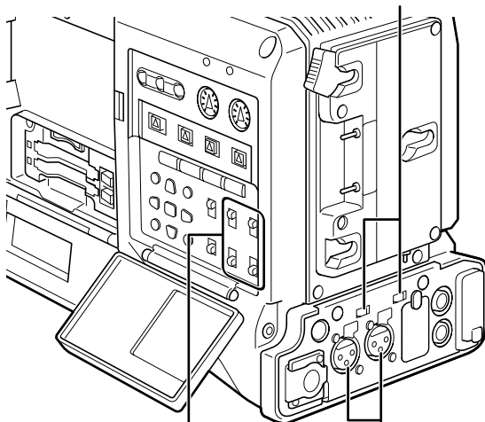
AUDIO IN Switch
