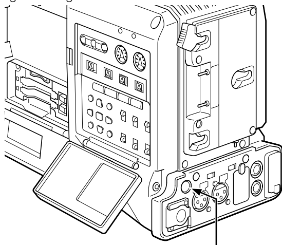
DC OUT connector
